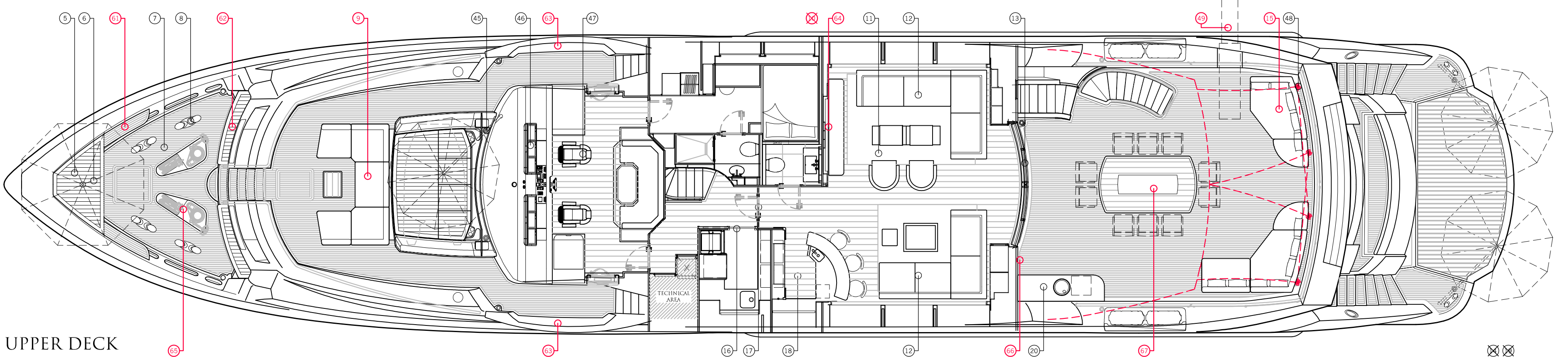
SKYDECK
